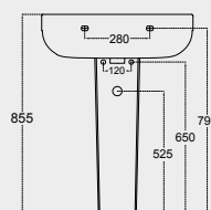
LAVABO (FO15) + COLONNA (M16) WASHBASIN (FO15) + PEDESTAL (M16)
