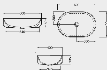
G60 LAVABO APPOGGIO OVALE 60 COUNTERTOP OVAL WASHBASIN 60
