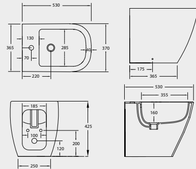
FA14 BIDET BACK TO WALL BIDET
