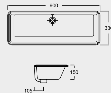
A 110 GEA LAVABO SOTTOPIANO 90x33x15 GEA UNDER COUNTER WASHBASIN 90x33x15
