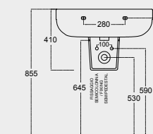
LAVABO (FO15) + SEMICOLONNA (M22) WASHBASIN (FO15) + SEMIPEDESTAL (M22)
